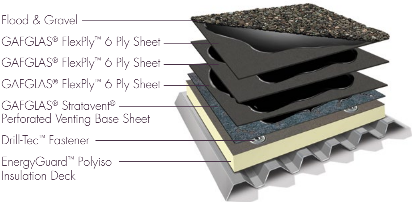
TYPICAL 4-PLY BUR SYSTEM WITH GAFGLAS® STRATAVENT®, FLEXPLY™ 6, FLOOD COAT, AND GRAVEL
