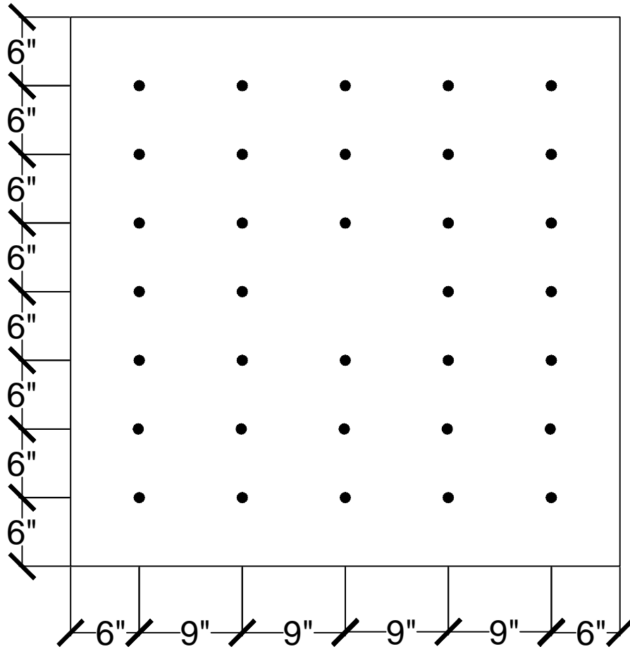
34 FASTENERS PER 4' x 4' BOARD
