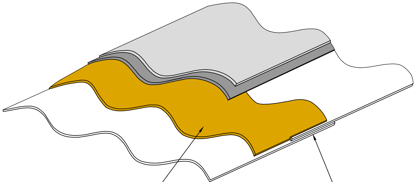
6" [152 mm] WIDE FLASHING GRADE SILICONE CENTERED OVER PANEL SEAM
